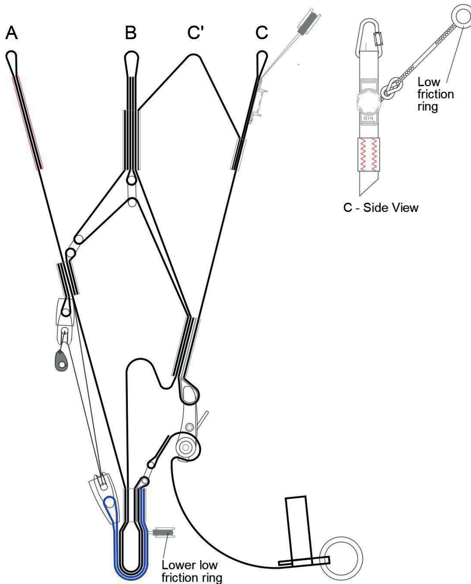
Figure: Vantage 3 riser
