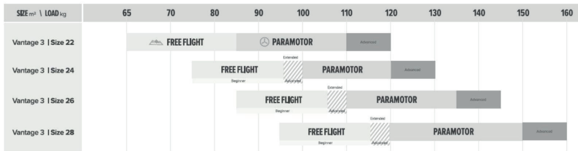
Figure: Vantage 3 load chart
