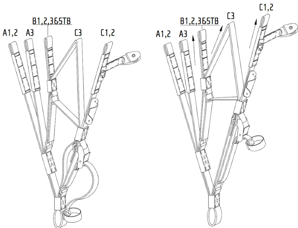
Figure: Osprey tandem-riser
