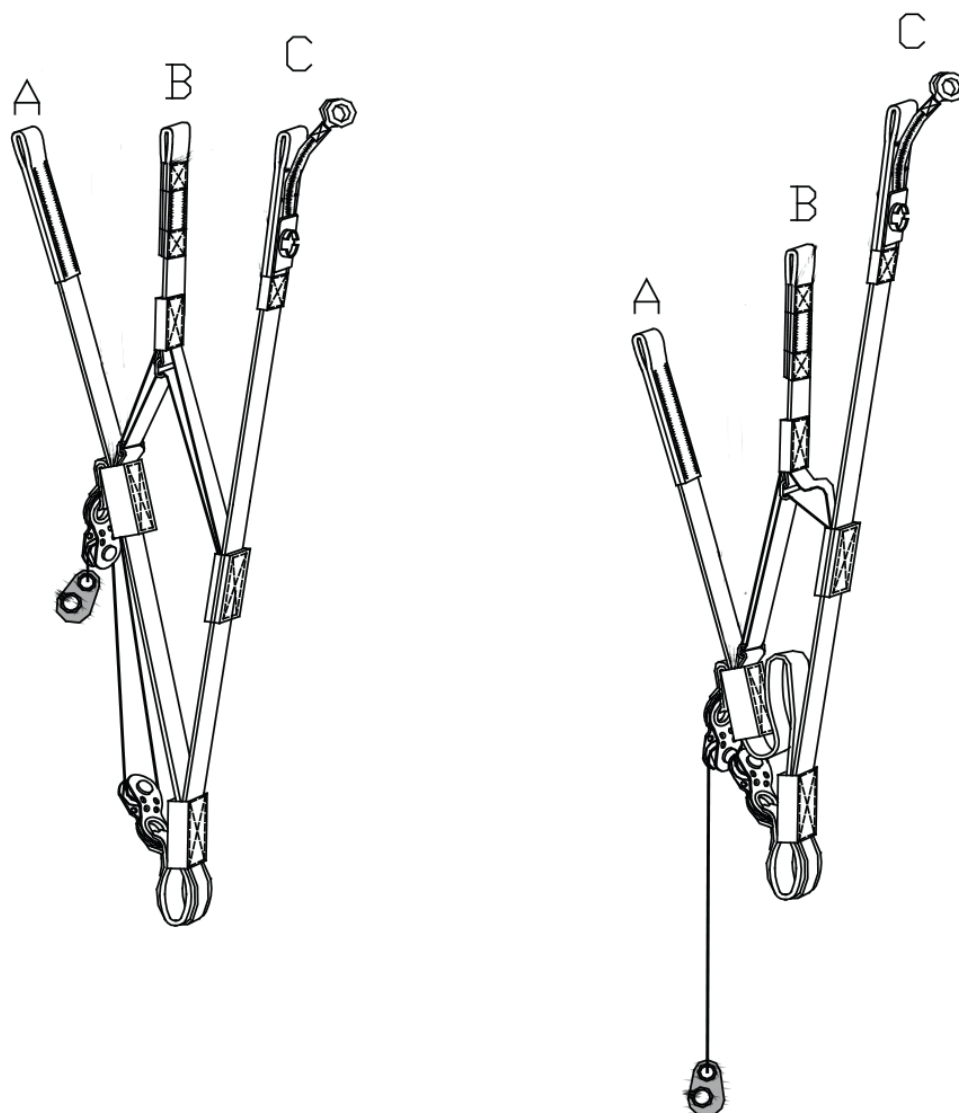
Figure: Griffin riser
